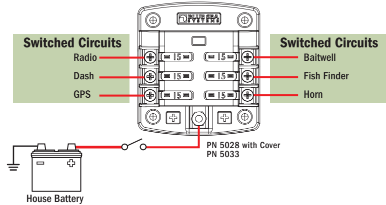
Example 6 Common Sourced Circuits
