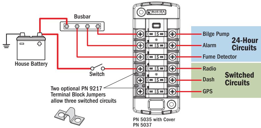
Example 3 Independent Sourced Circuits, 3 Common Sourced Circuits
